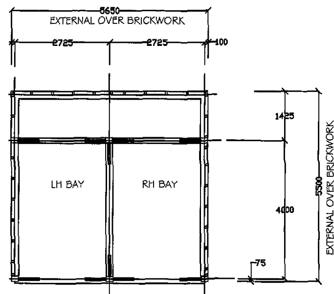
FLOOR PLAN
