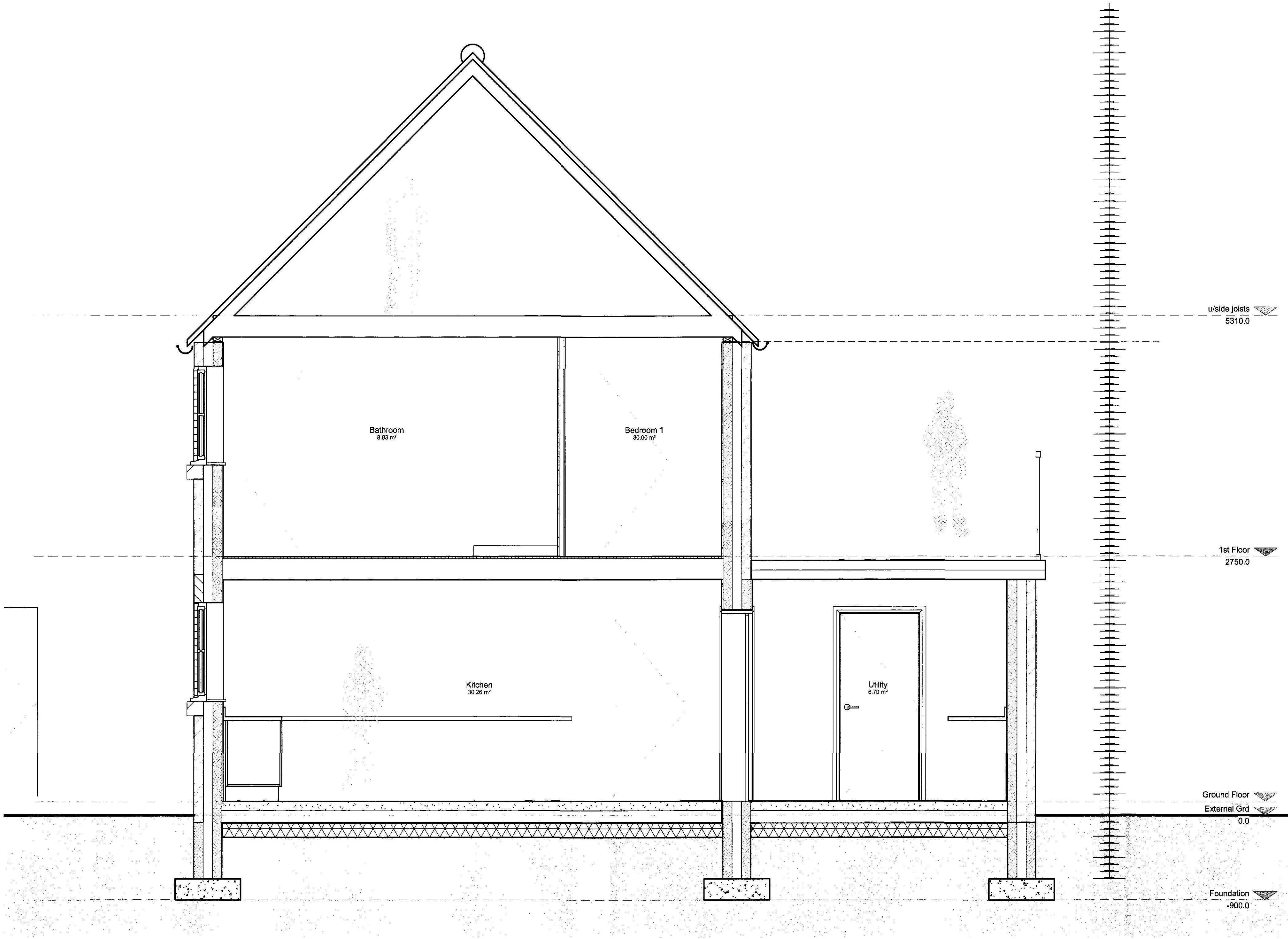
2 Section thro' Kitchen 1:25
