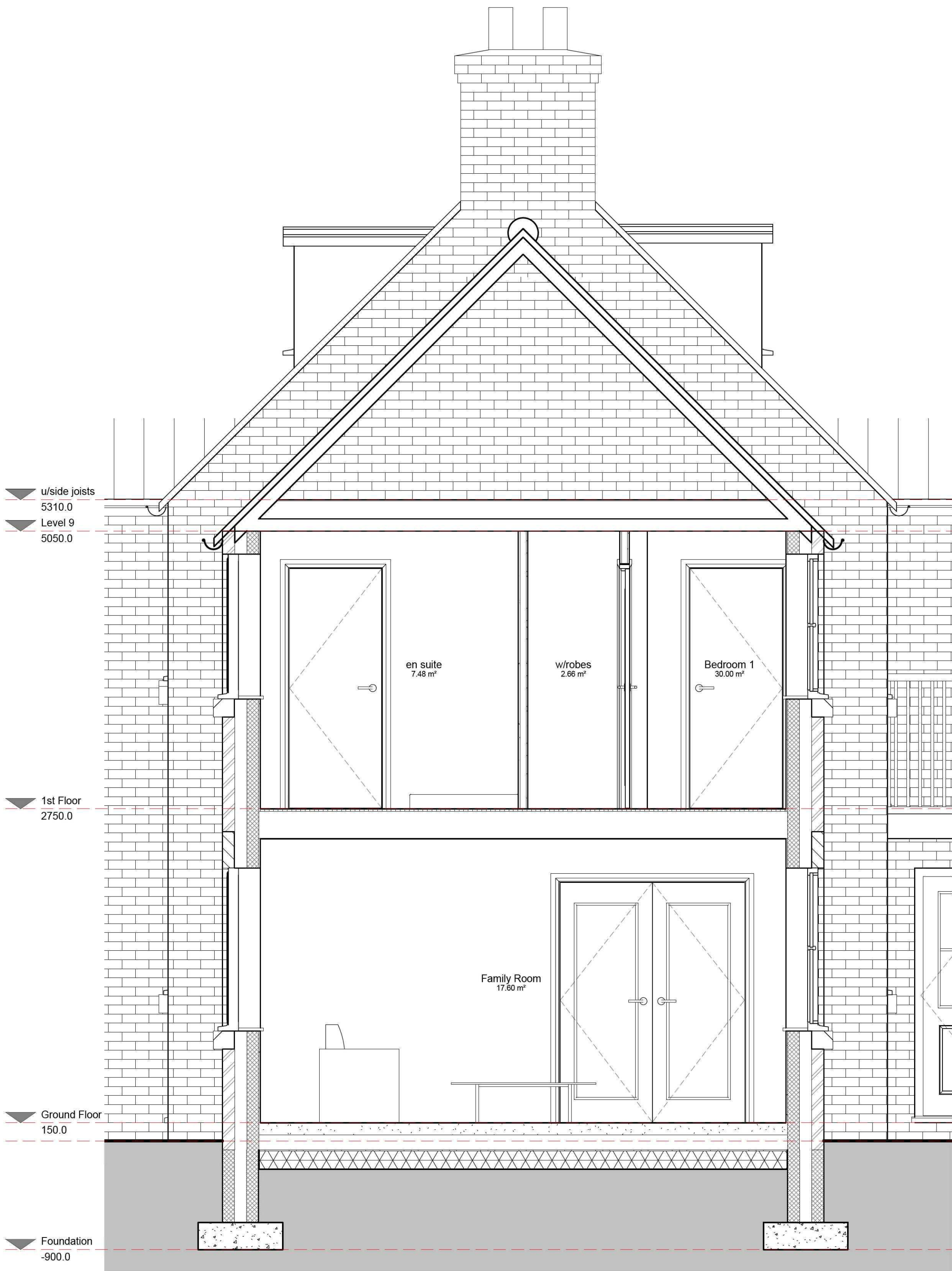
1 Section thro' Family Room 1 : 25
