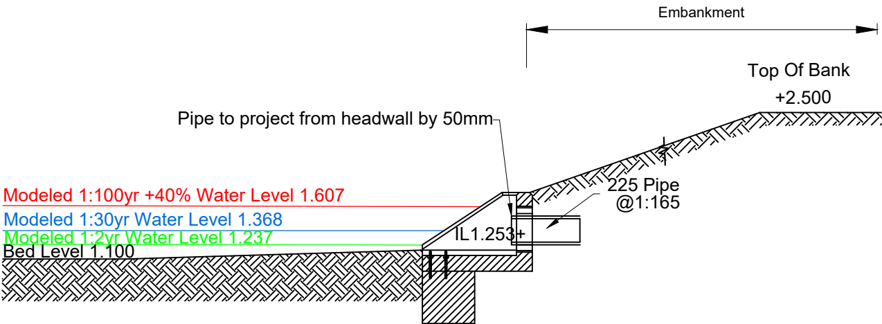
Section (1:50) HEADWALL OUTFALL 4
