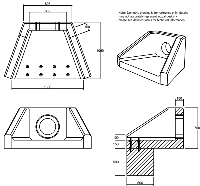
HEADWALL DETAIL 4 SFA6 A HEADWALL
