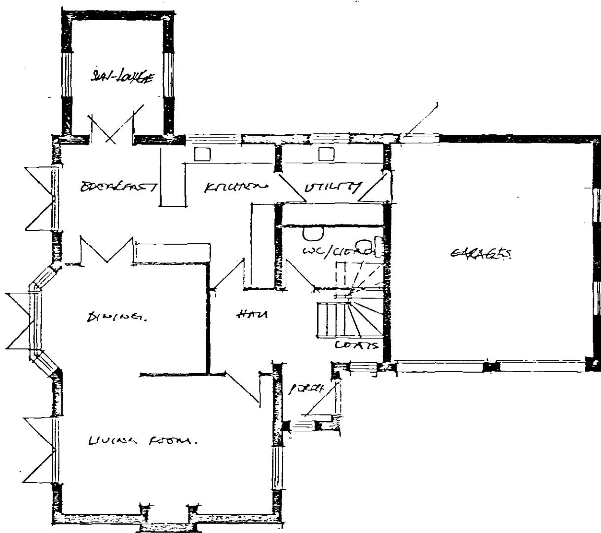
GROUND FLOOR
