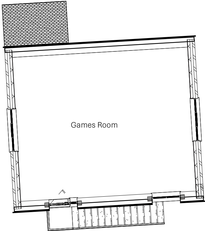
1 EP-301.1 Rev2 FIRST FLOOR (EXISTING) Outhouse 1 : 100
