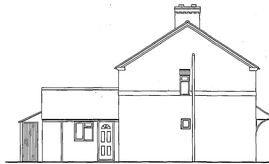
SOUTH - WEST ELEVATION (EXISTING)
