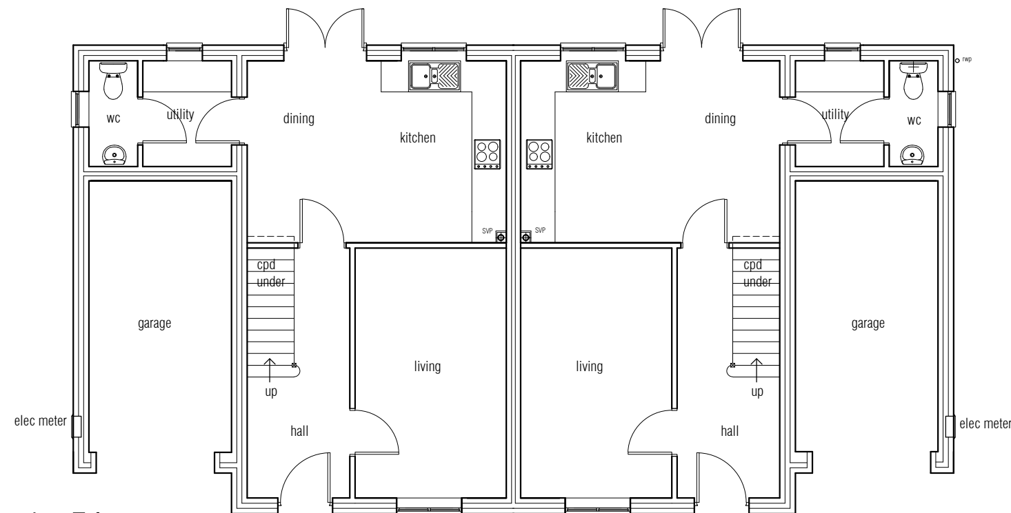
Ground Floor
