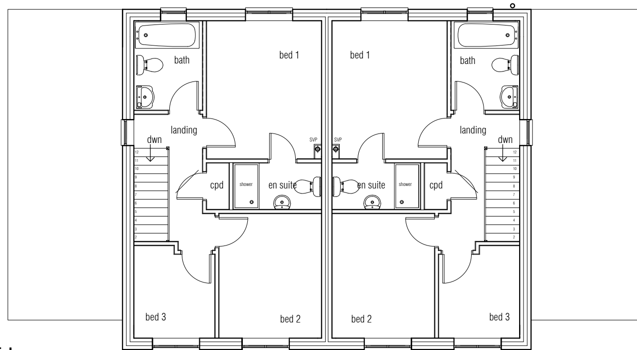
First Floor
