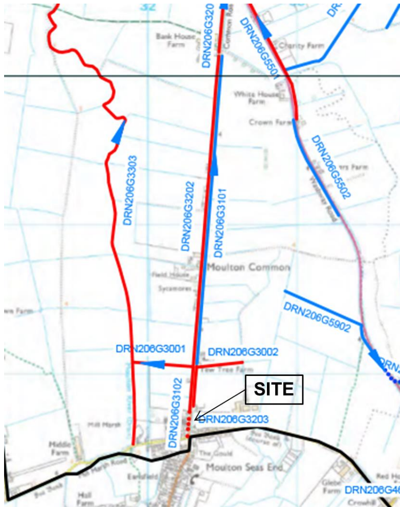
PLAN SHOWING SITE LEVELS
