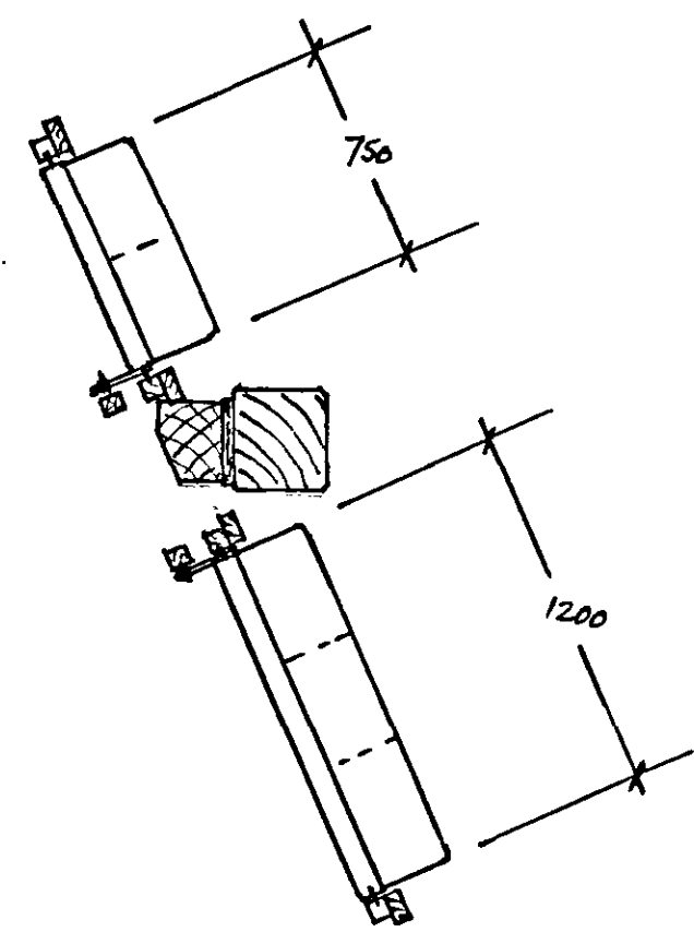
SECTION AT SHUTTERS
