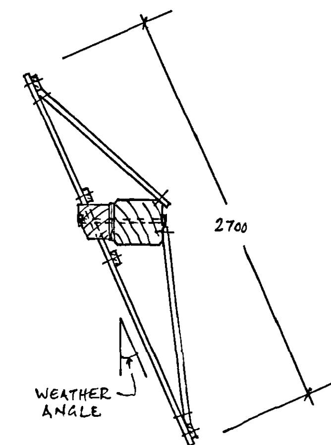
SECTION AT SAILBAR 6 SETS BACKSTAYS REQ'D AS SHOWN FOR EACH SAIL AT 'S'
