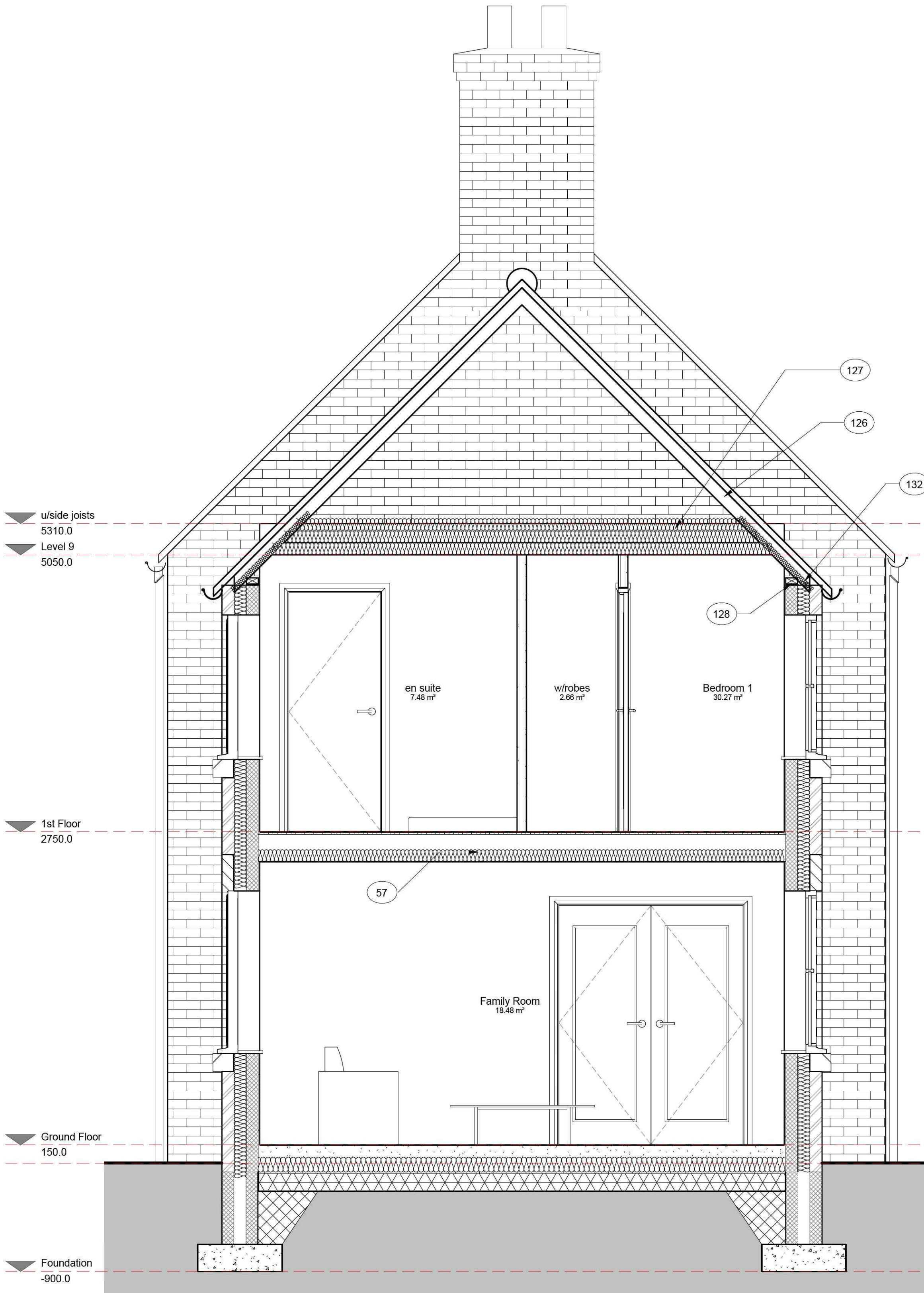
1 Section thro' Family Room 1 : 25
