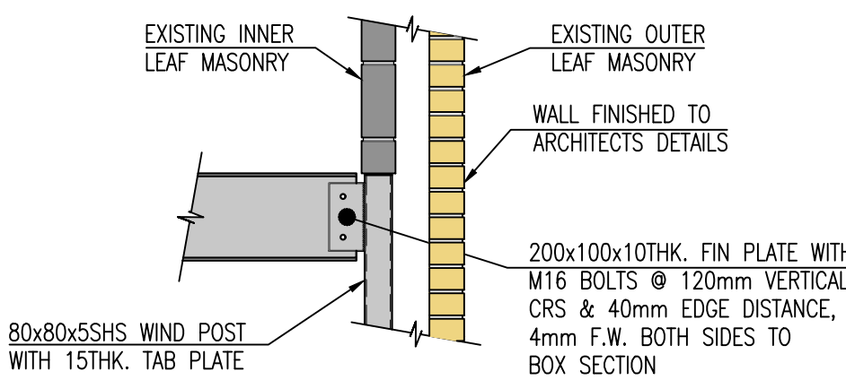
ELEVATION DETAIL ON POST
