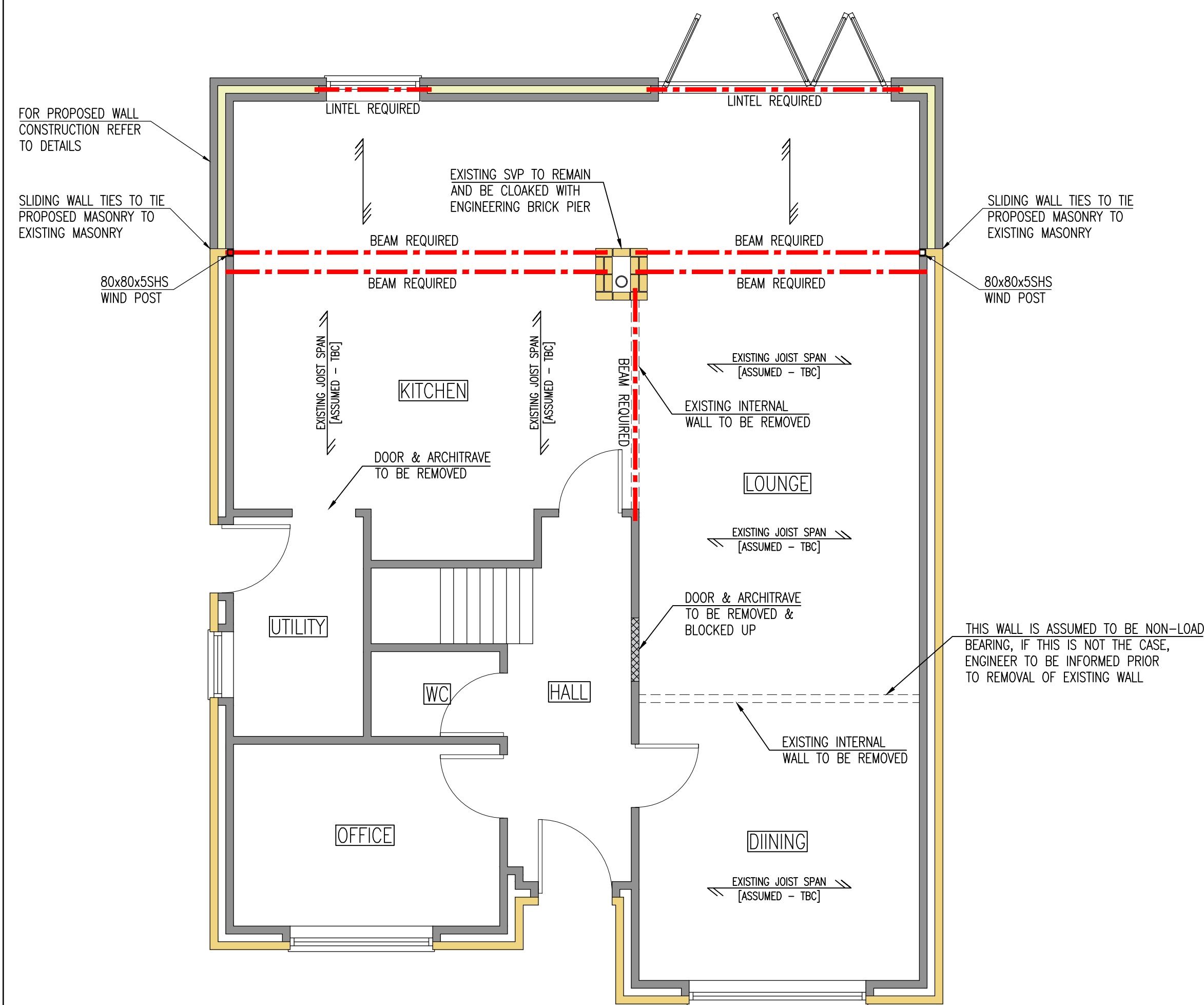
PROPOSED SUPERSTRUCTURE ARRANGEMENT SCALE 1:50
