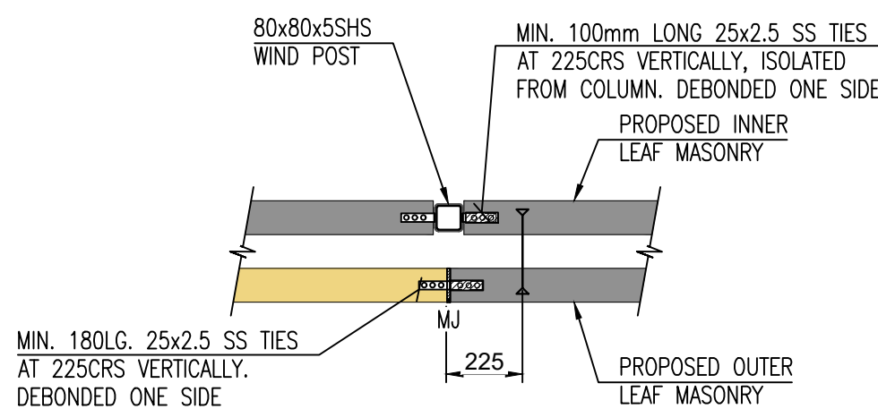
PLAN ON WIND POST / MOVEMENT JOINT DETAIL
