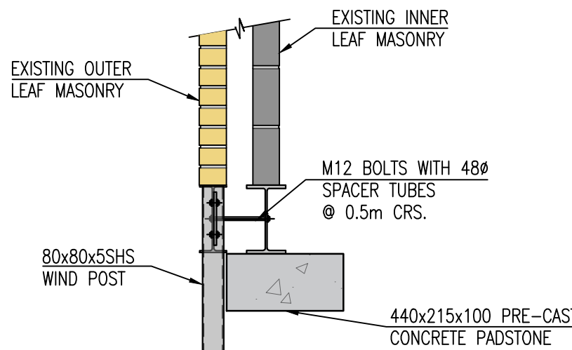
SECTION THROUGH BEAM END BEARING
