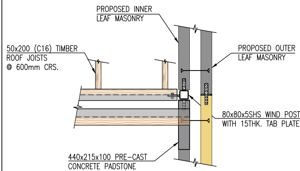
PLAN DETAIL ON POST
