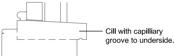
Vertical Section
