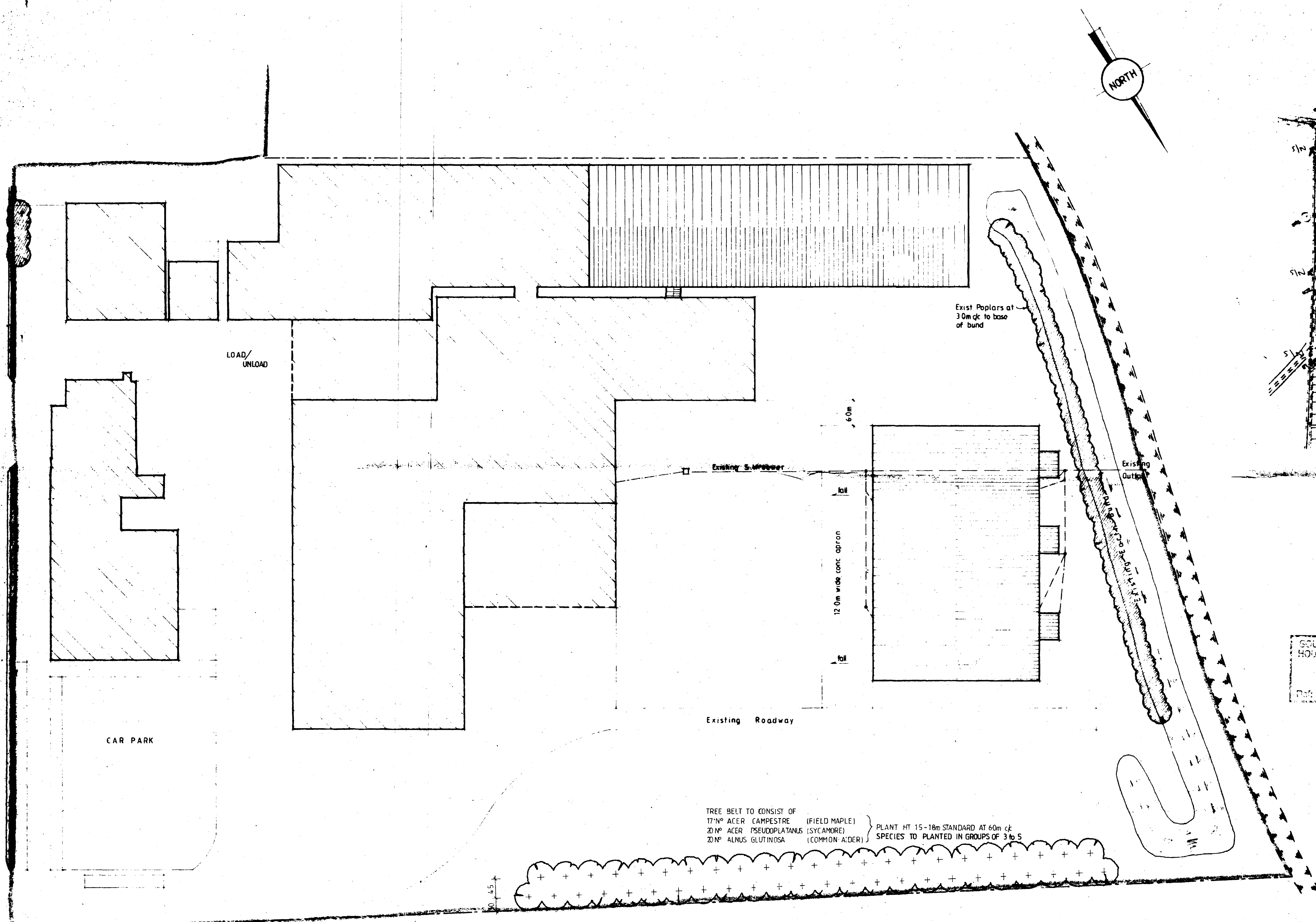
BLOCK PLAN 1:500
