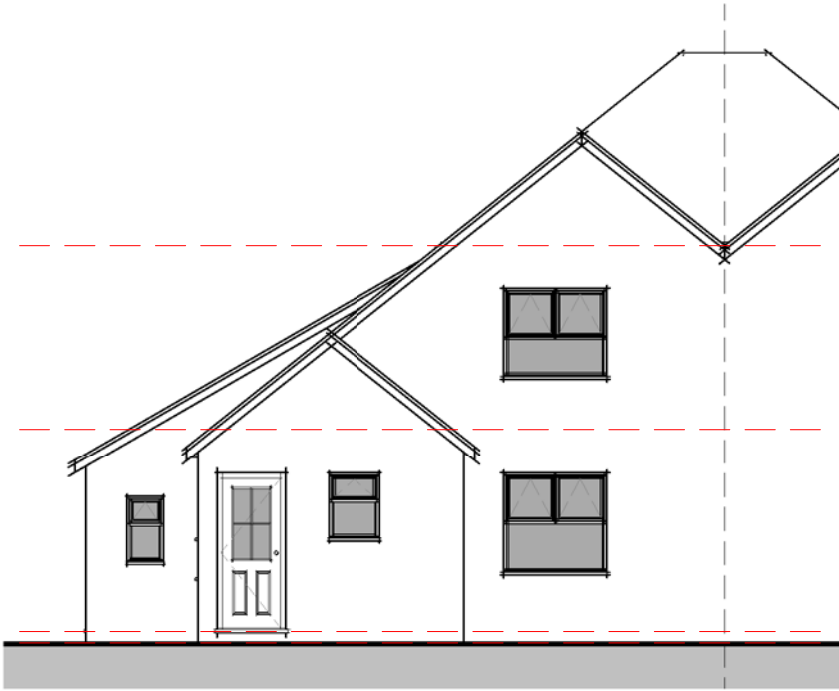
Elevation 03 - Rear 1 : 100
