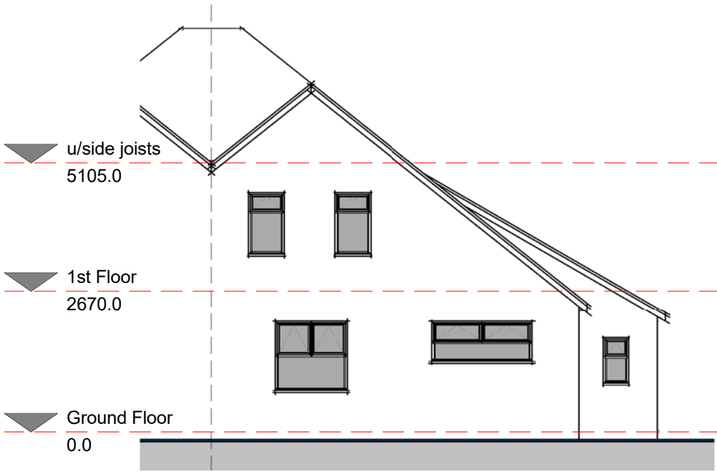
Elevation 01 - Front 1 : 100
