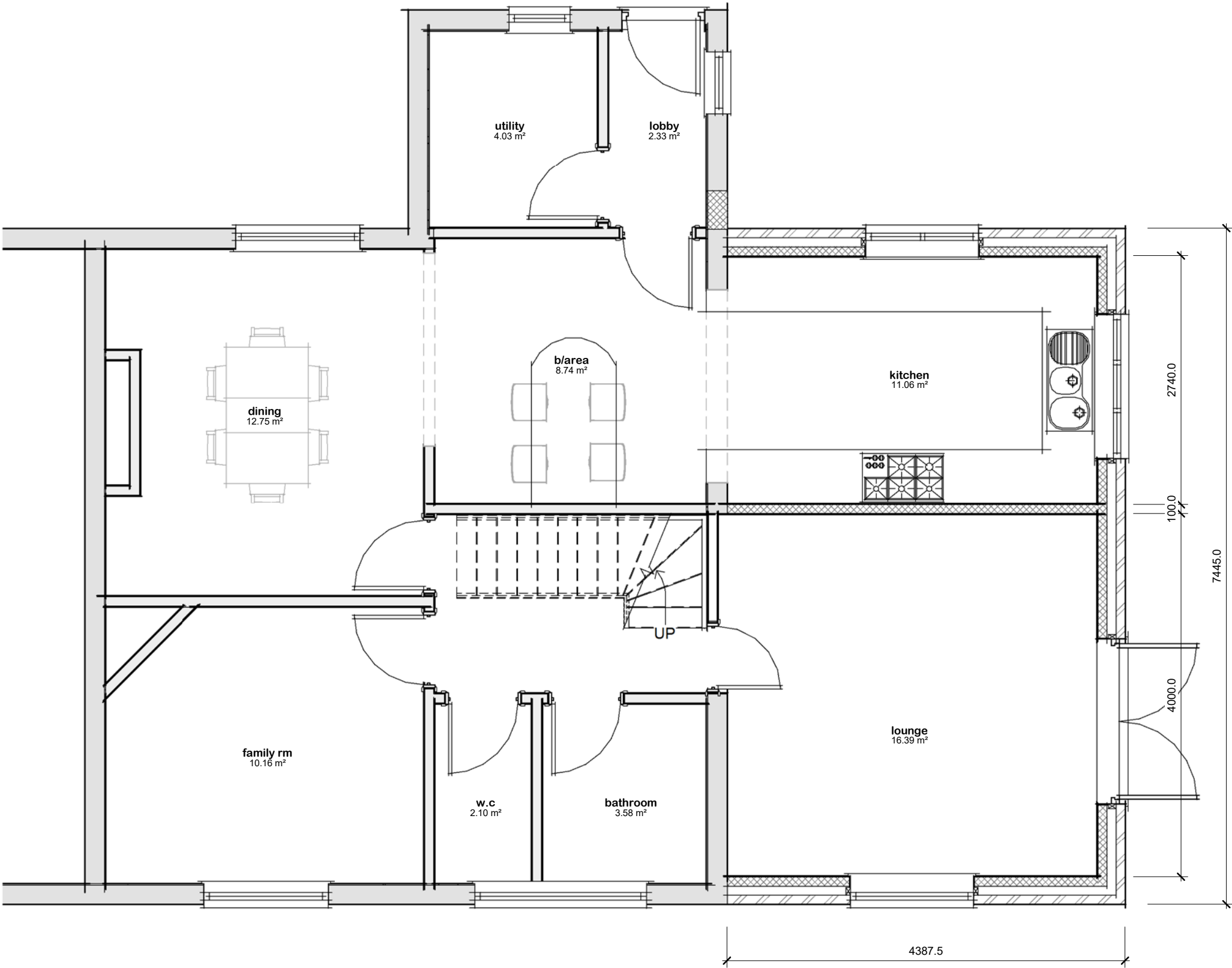
Plan 01 - Ground 1 : 50
