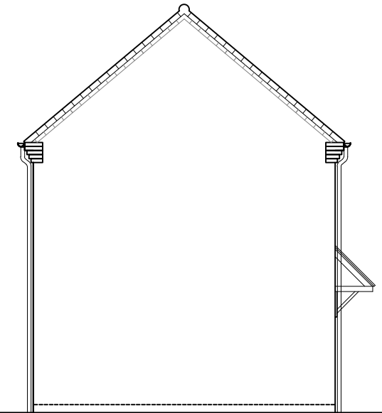
SIDE ELEVATION
