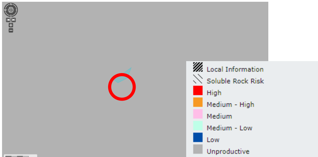
Figure 6 – Groundwater vulnerability map, site highlighted.
