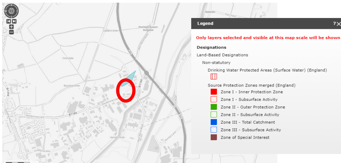
Figure 7 – Groundwater source protection zones, site highlighted.
