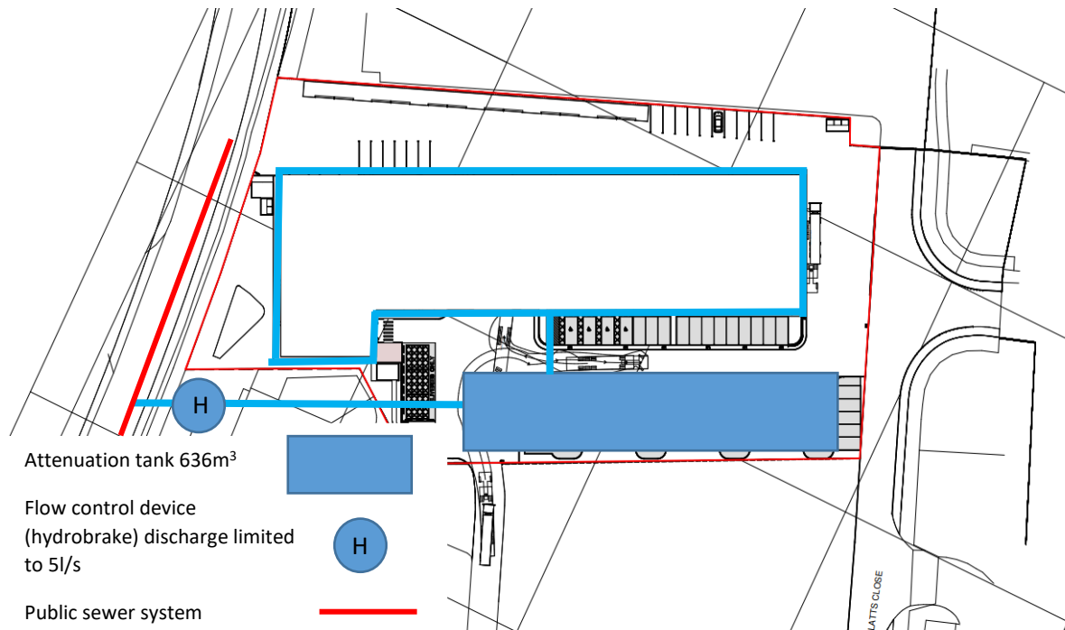
Figure 11 – Drainage layout.
