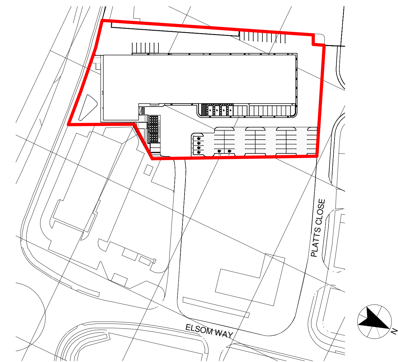
Proposed Site Location Plan 1:1250
