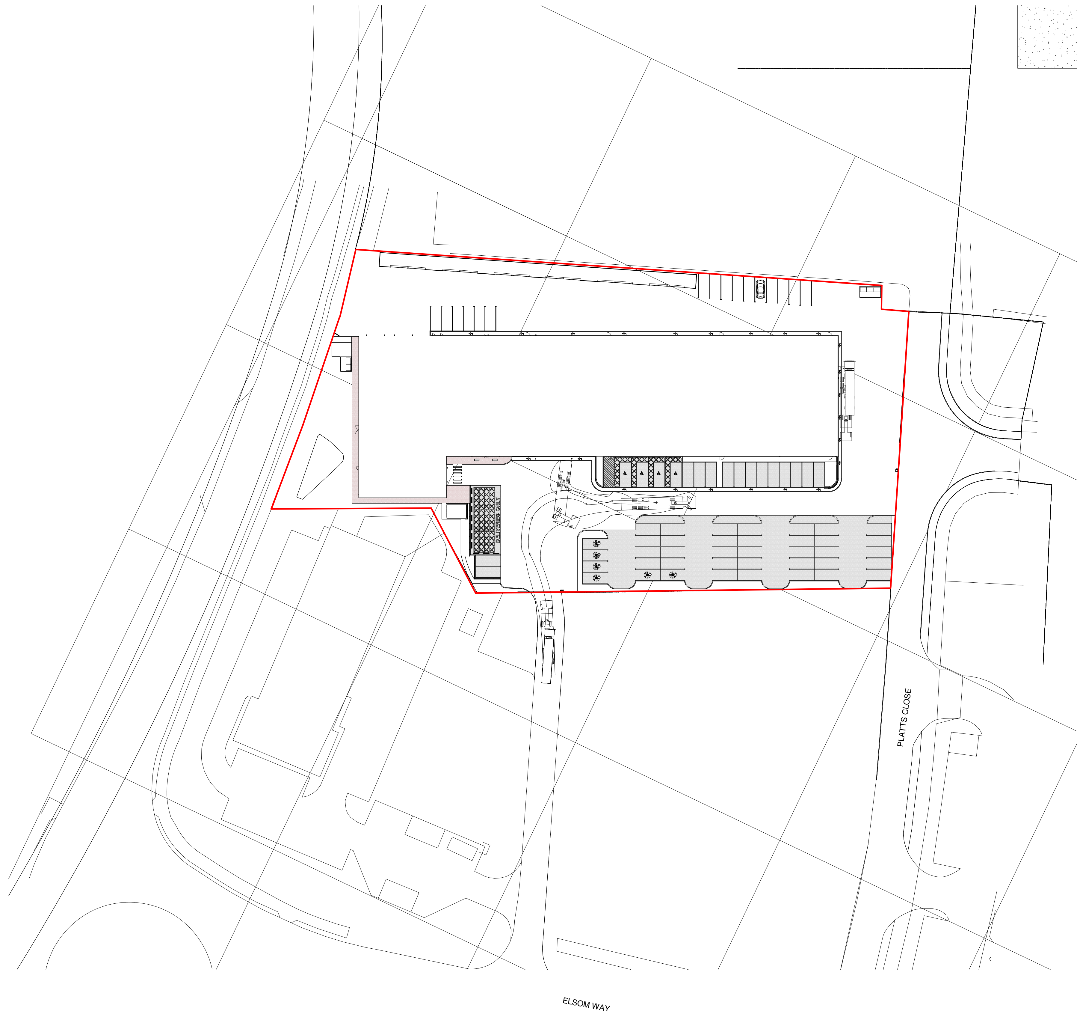
Proposed Site Plan 1:500
