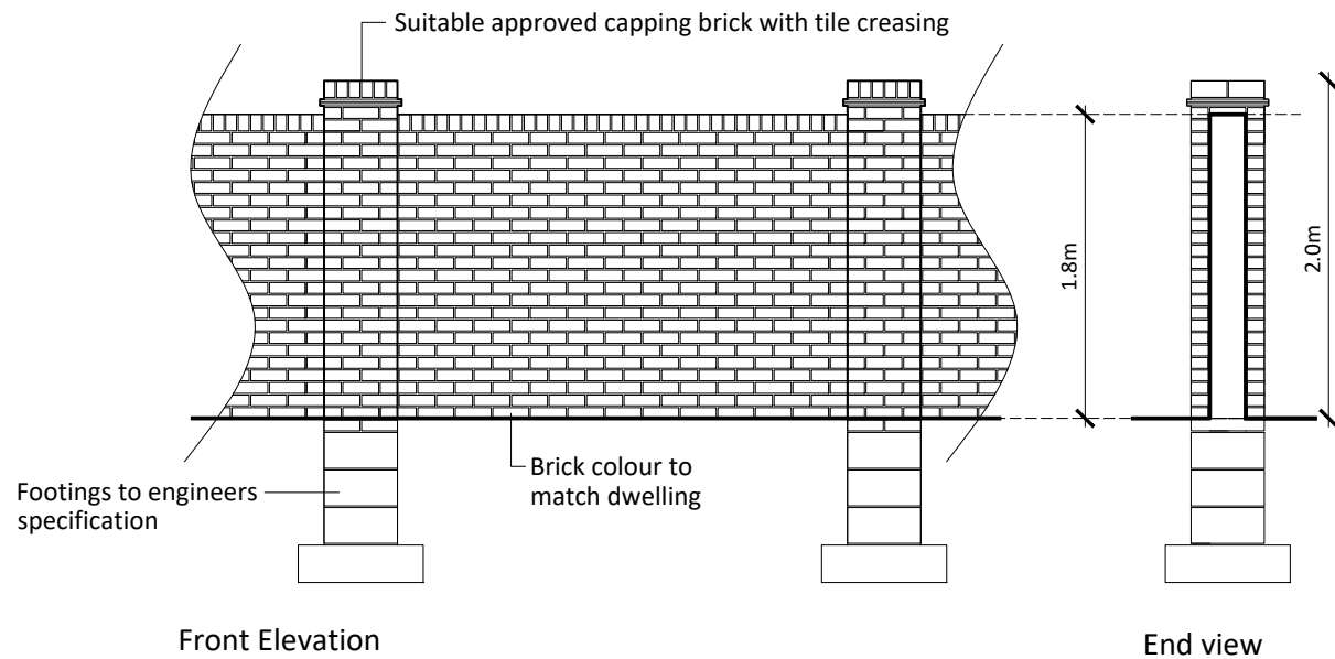
1.8m high brick wall with piers
