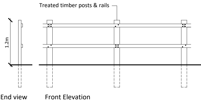
1.2m high timber post & rail fence
