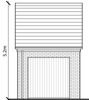
Front Elevation
