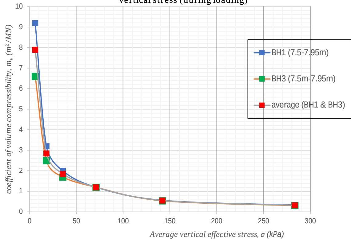
Figure 7: Deep TFD very soft peaty silt/clay - m_v values against vertical stress (during loading)
