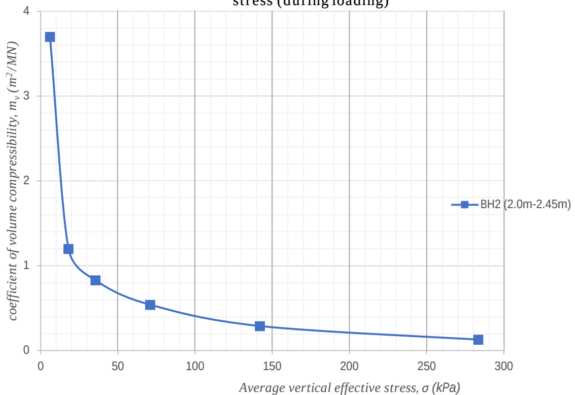
Figure 8: Shallow very soft TFD silt/clay - m_v values against vertical stress (during loading)
