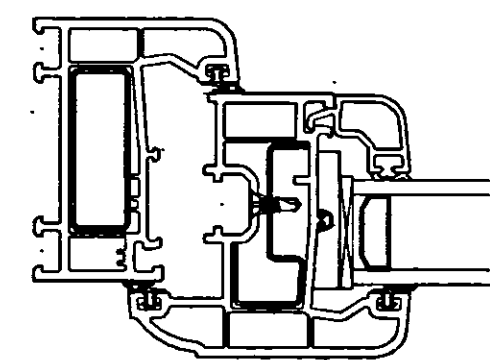
TYPICAL SECTION THROUGH JAMB 1:2
