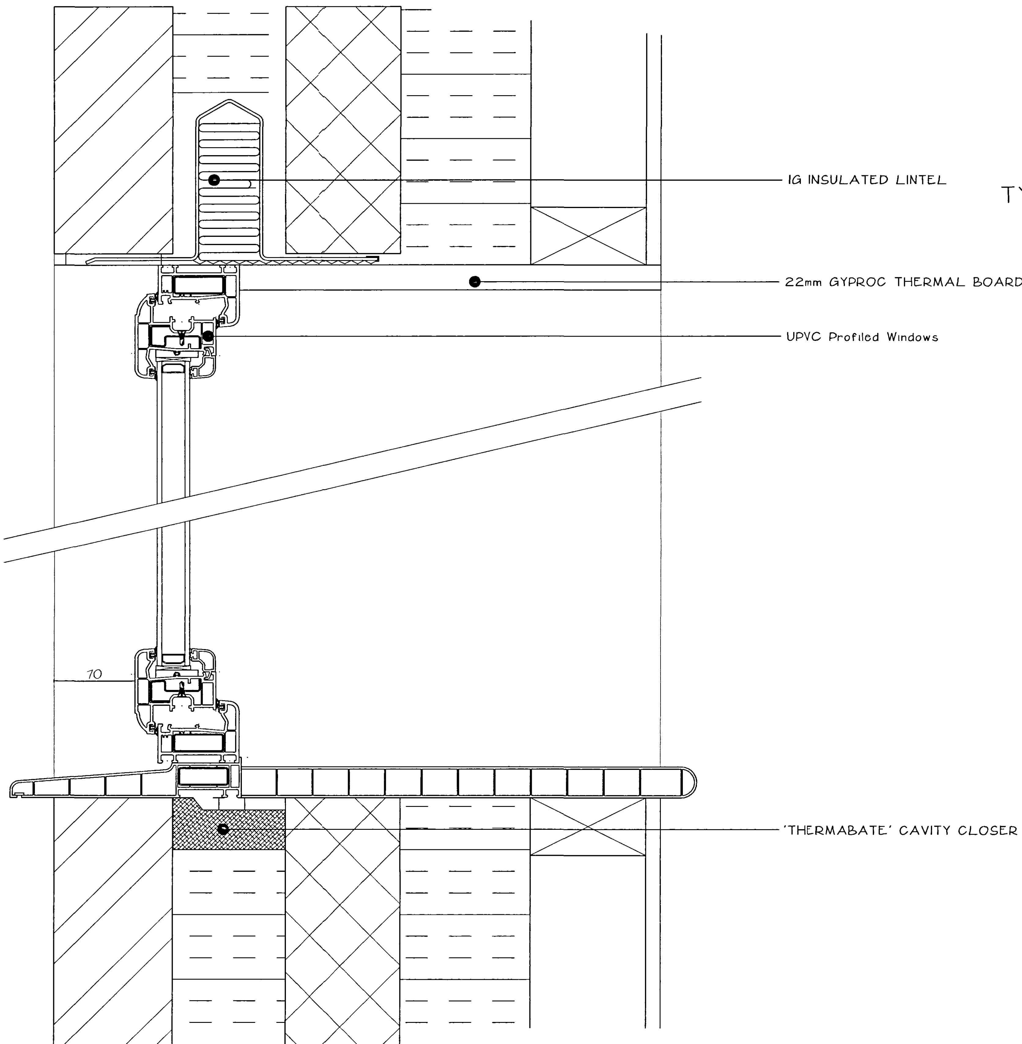
TYPICAL SECTION THROUGH CASEMENT WINDOW 1:2
