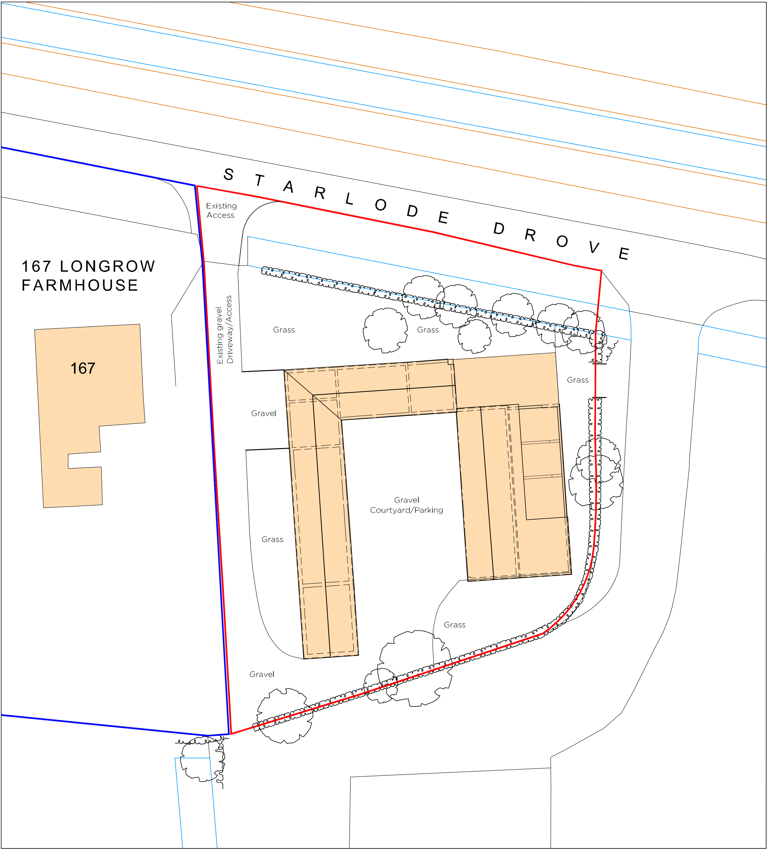
Existing Site Layout Scale 1:200
