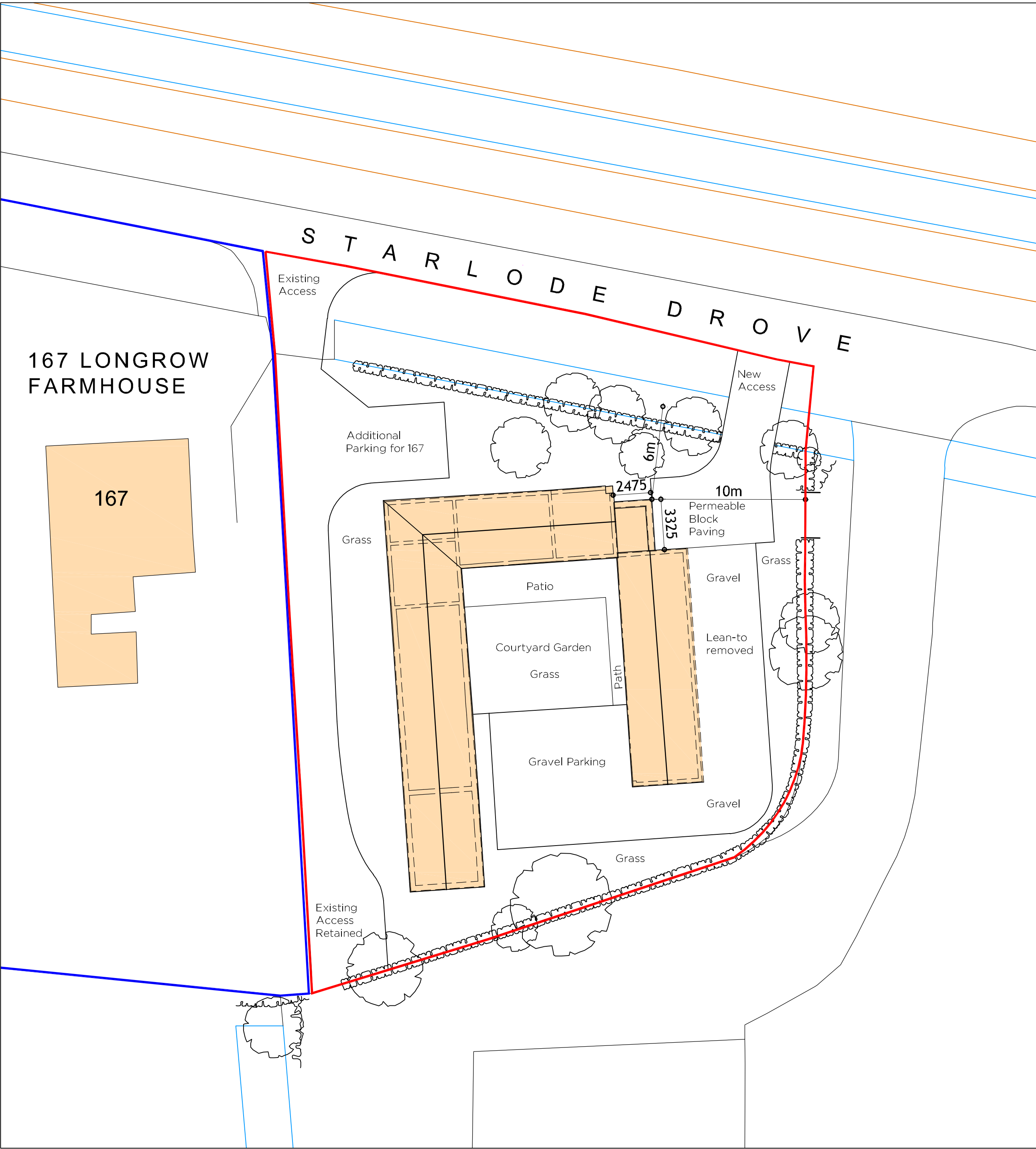
Proposed Site Layout Scale 1:200
