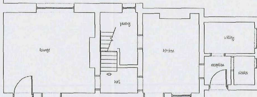
EXISTING GROUND FLOOR PLAN
