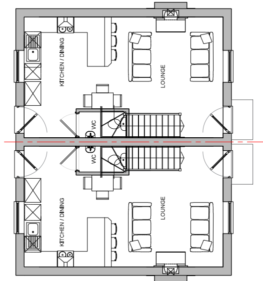
GROUND FLOOR GENERAL ARRANGEMENT PLAN SCALE 1:50 2 BEDROOM 3 PERSON SEMI-DETACHED GF - 33.5m 2 (per unit) 1st - 33.5m 2 (per unit) SCALE 1:50 SCALE 1:1
