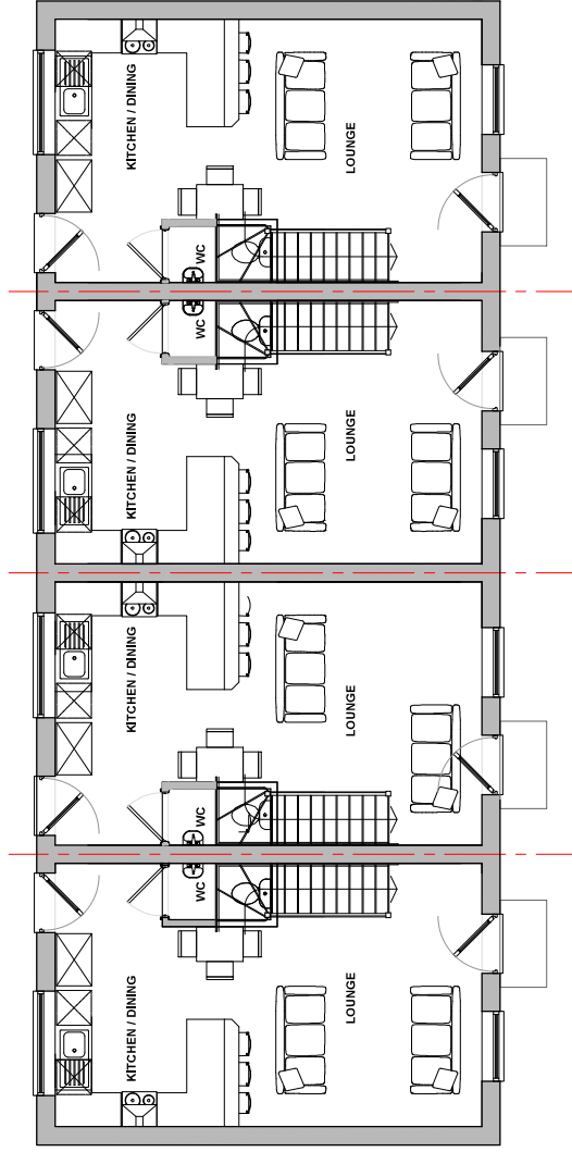
GROUND FLOOR GENERAL ARRANGEMENT PLAN SCALE 1:50 2 BEDROOM 3 PERSON TERRACE GF - 33m 2 (per unit) 1st - 33m 2 (per unit) SCALE 1:50 SCALE 1:1
