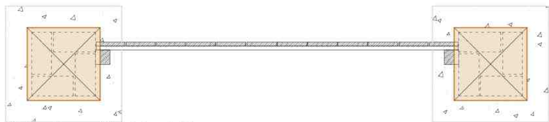
Timber Fence with brick pier Plan
