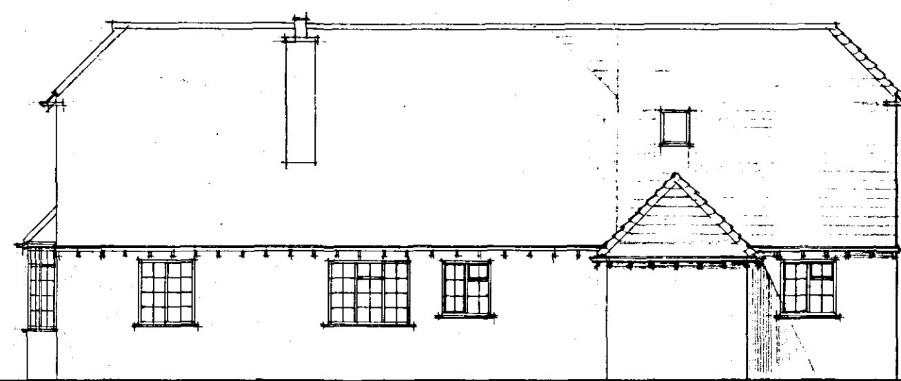
SOUTH ELEVATION
