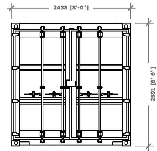
Elevation C
