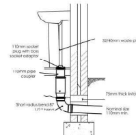
INTERNAL WASTE PIPE CONNECTION
