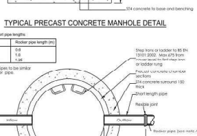
TYPICAL PRECAST CONCRETE MANHOLE DETAIL
