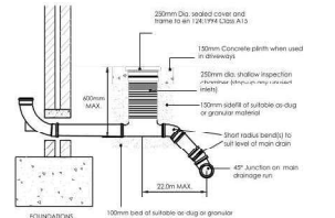
SHALLOW INSPECTION CHAMBER
