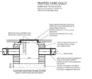
TRAPPED YARD GULLY
