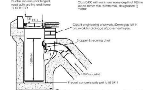
PRECAST ROAD GULLY
