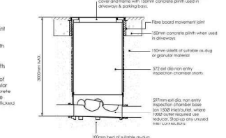
1.2m x 3.0m DEEP NON ENTRY INSPECTION CHAMBER
