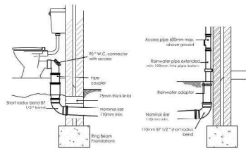
W.C. DIRECT TO DRAIN
