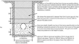
CLASS B+ BEDDING FACTOR 1.2 FOR USE WITH CONCRETE & CLAY PIPES
