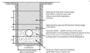
BEDDING DETAIL FOR UPVC PIPES
