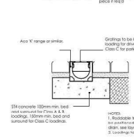
'A/C' DRAINAGE DETAIL
