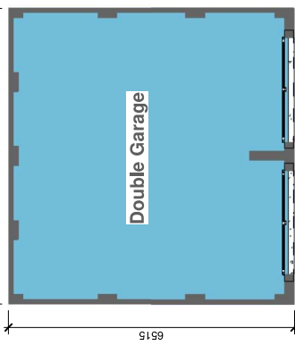
6 Ground Floor (Twin) 1 : 100
