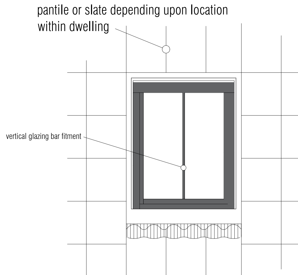
plan view onto conservation type rooflight colour to be anthracite grey ( factory finish )
