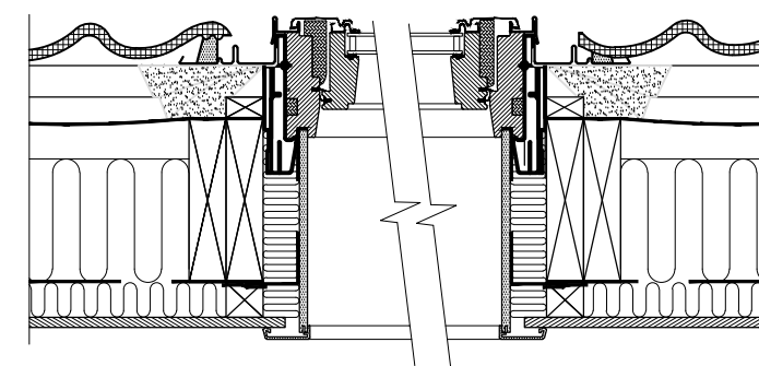
vertical section thro rooflight
