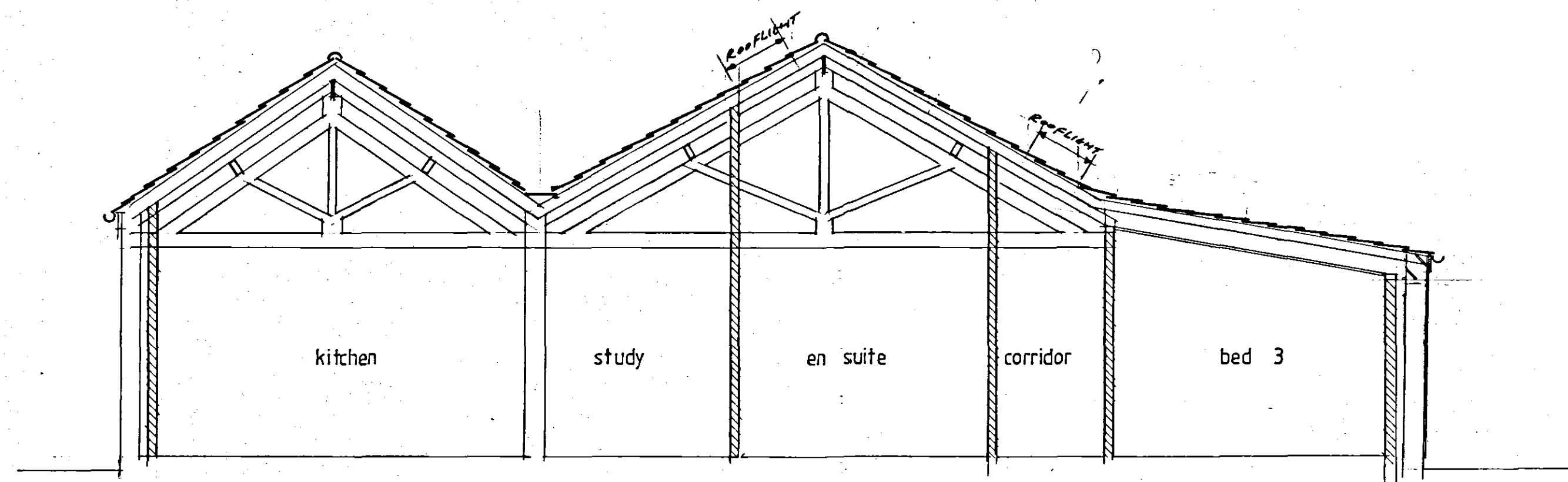
section 1-50
