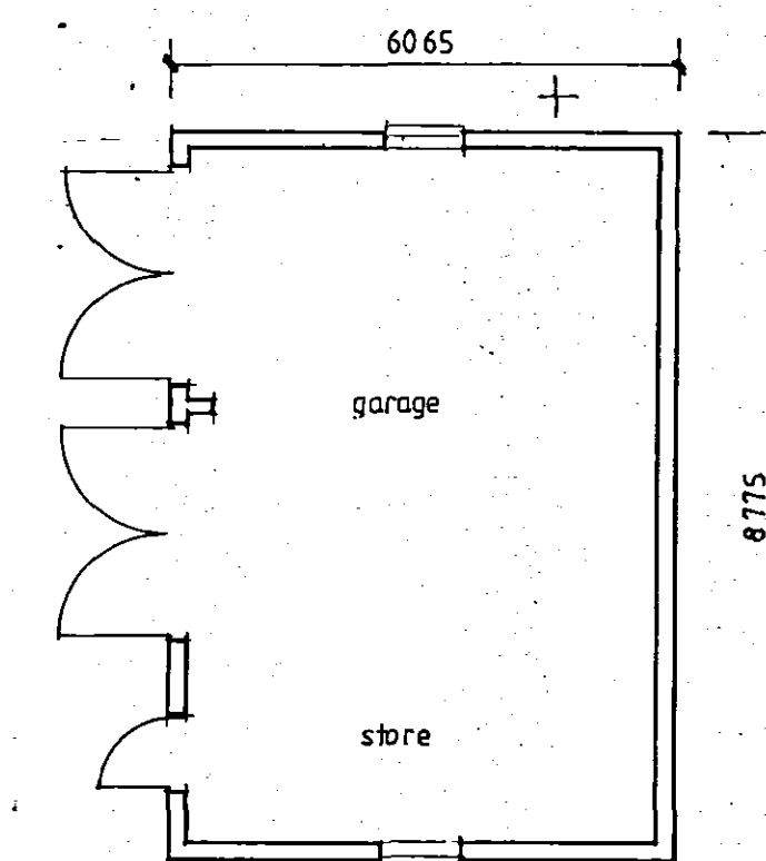
plan 1-100
