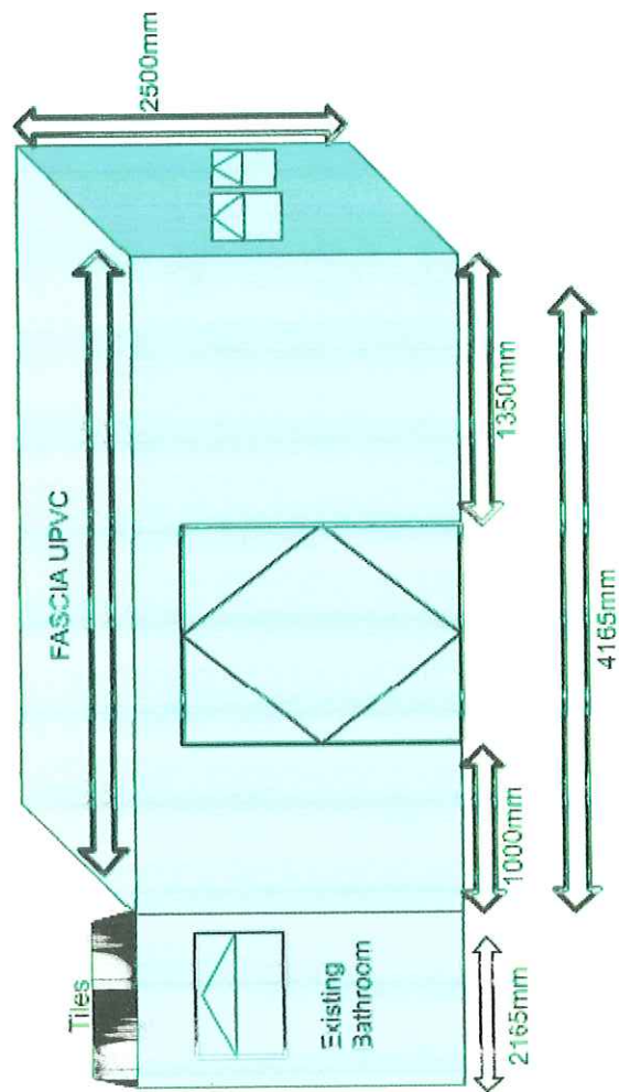
Rear View
