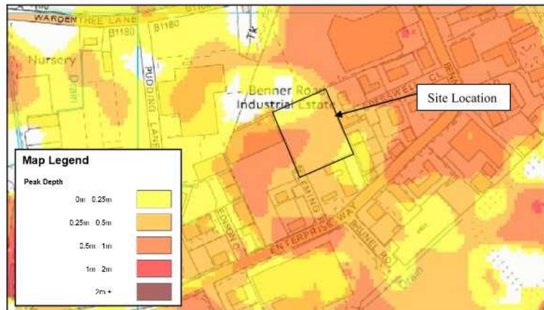
Figure 3 – SFRA 2116 Residual Peak Depth Map during the 1% fluvial and 0.5% tidal Annual Probability Event
