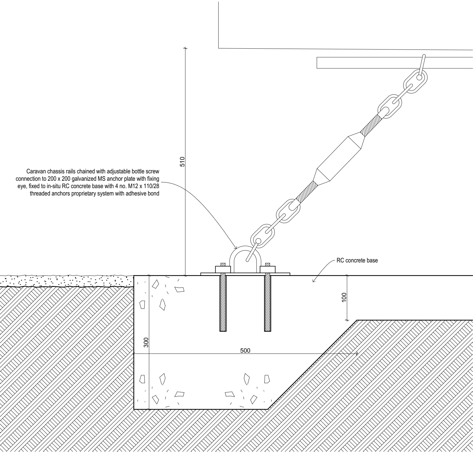
Section through fixing plate and caravan slab
