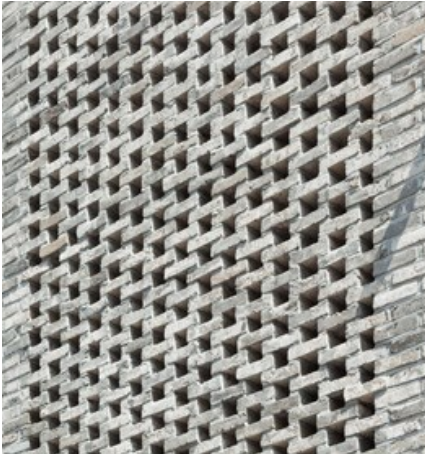
Example Perforated Brickwork
