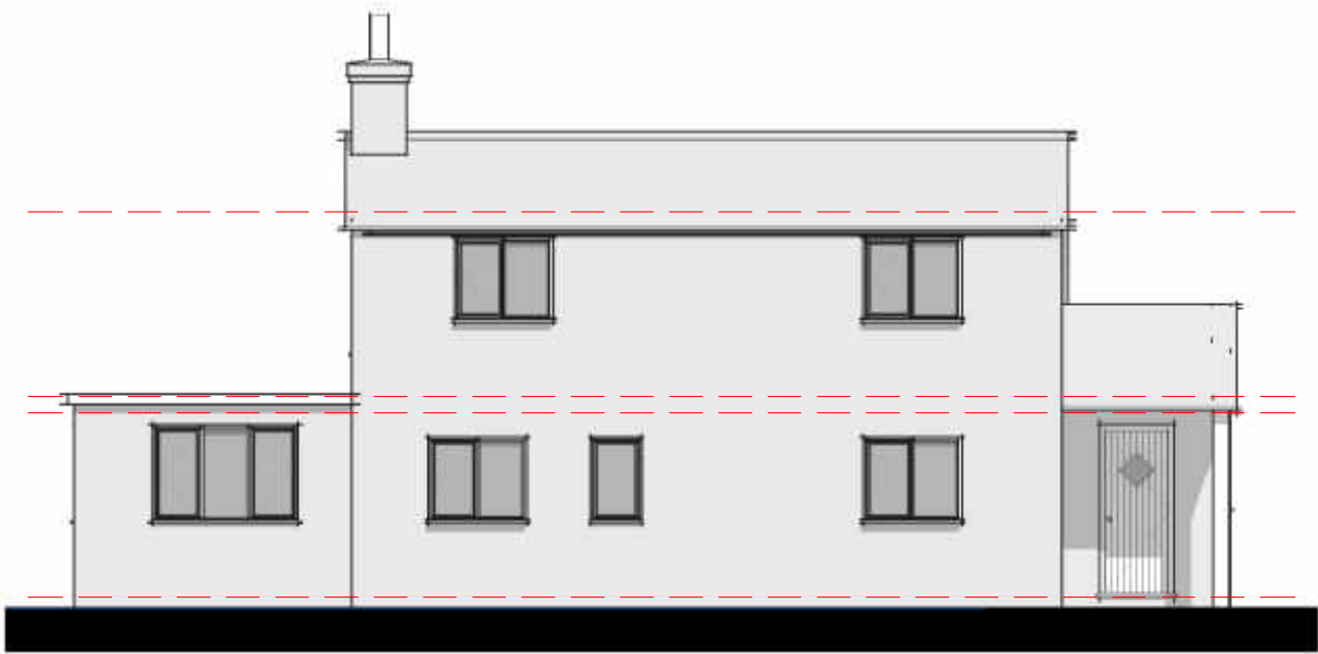
Elevation 01 - Front 1 : 100
