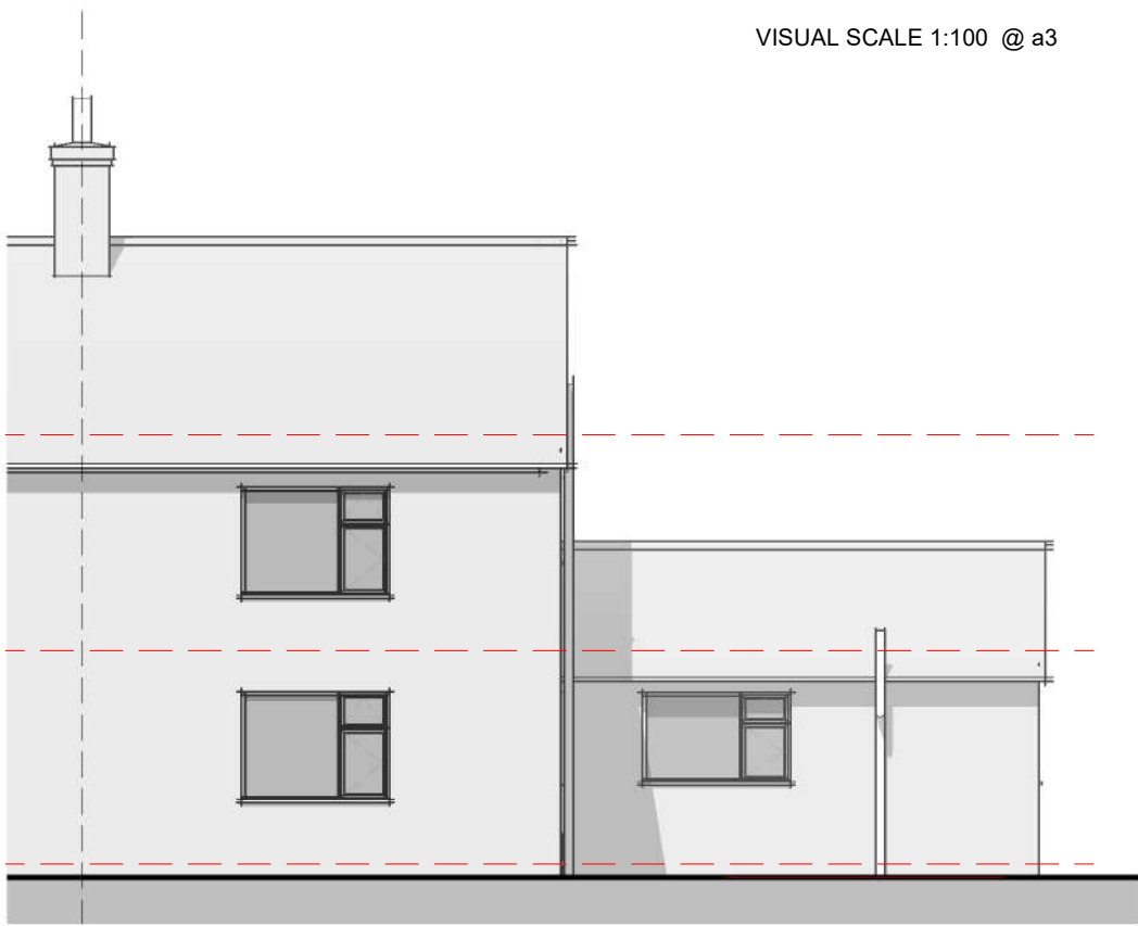
Elevation 01 - Front 1 : 100
