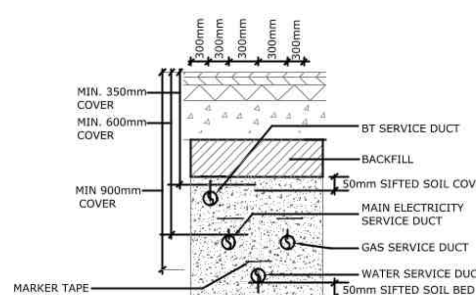
DETAIL C TYPICAL SECTION ON COMBINED SERVICES TRENCH (NTS)
