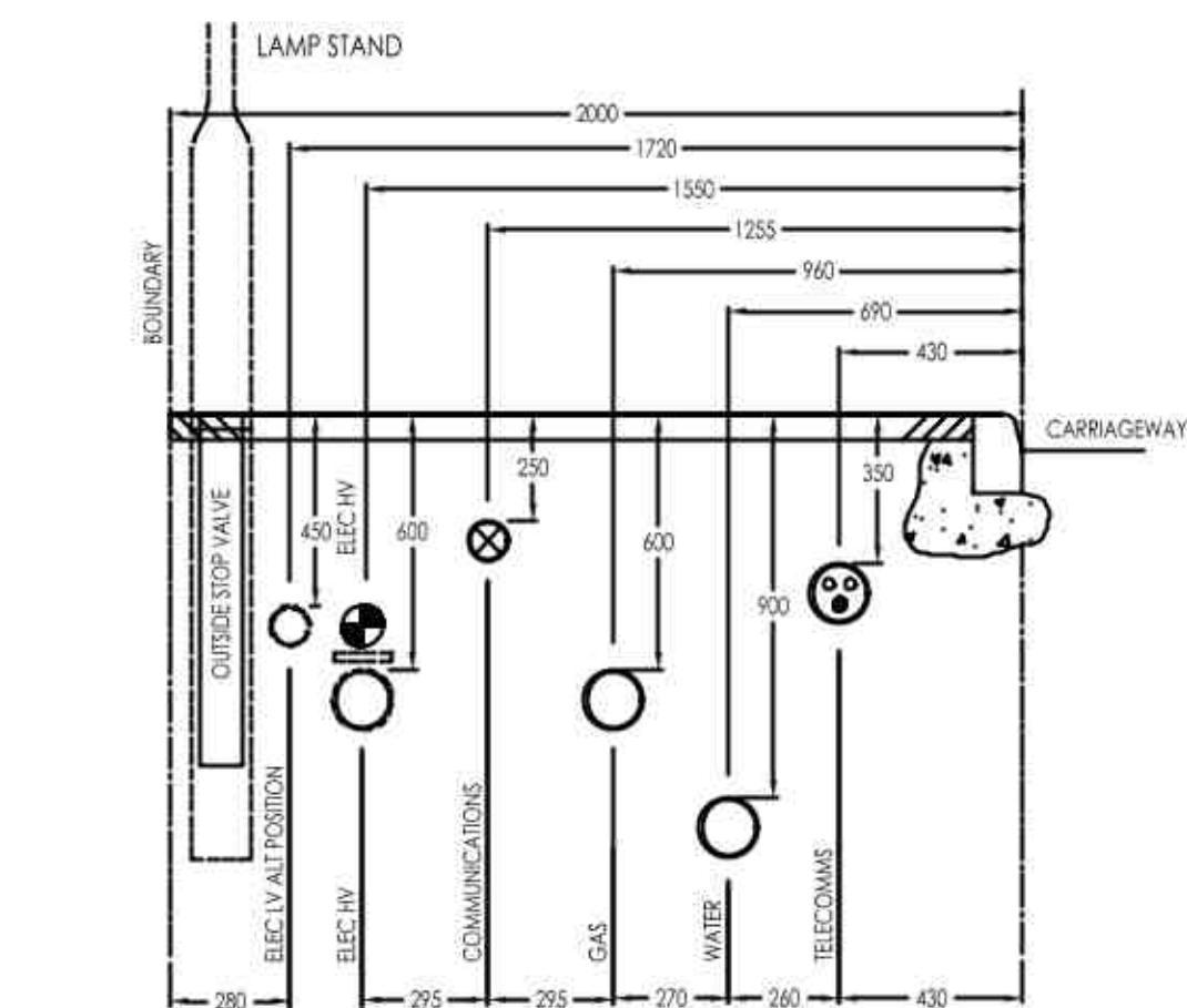
DETAIL C: TYPICAL SERVICES IN A 2m FOOTWAY
