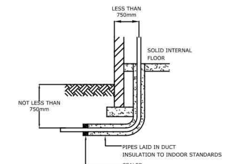
DETAIL B TYPICAL MAINS COLD WATER SERVICE ENTRY DETAIL
