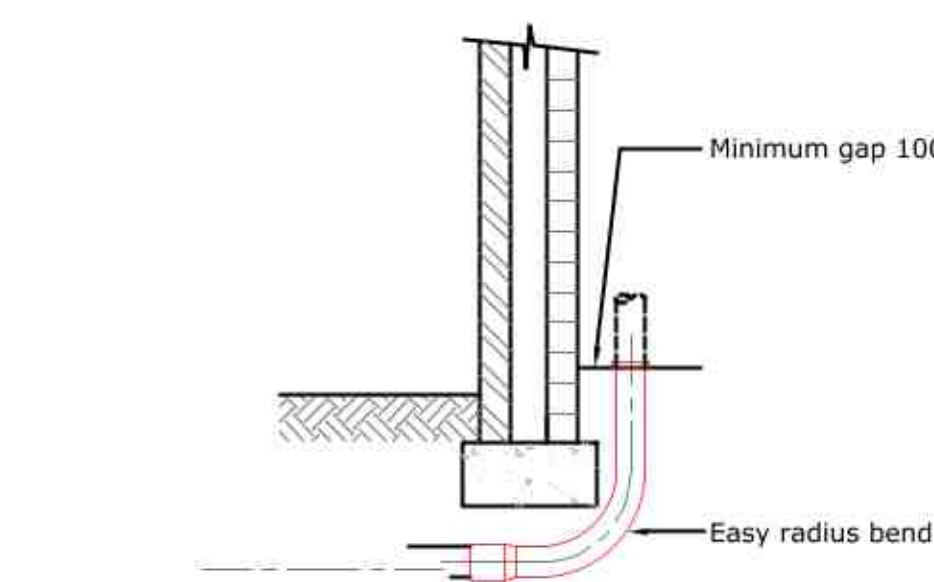
DETAIL A: TYPICAL INCOMING ELECTRICAL SERVICE ENTRY DETAIL
