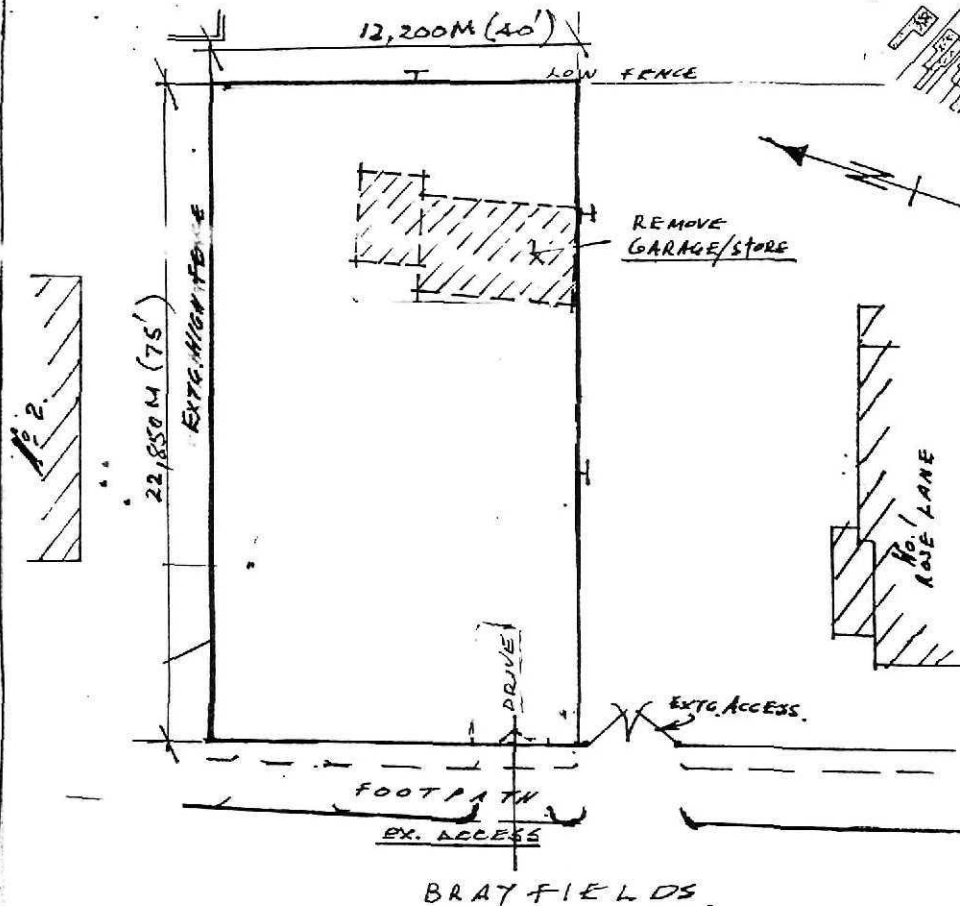
BLOCK PLAN SCALE 1:250
