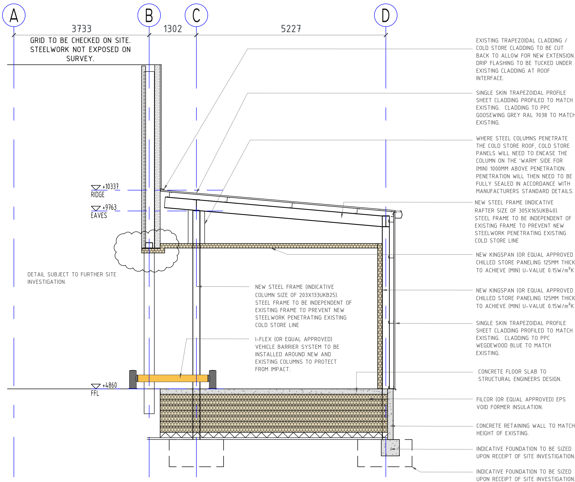
SECTION B-B SCALE 1:50@A1
