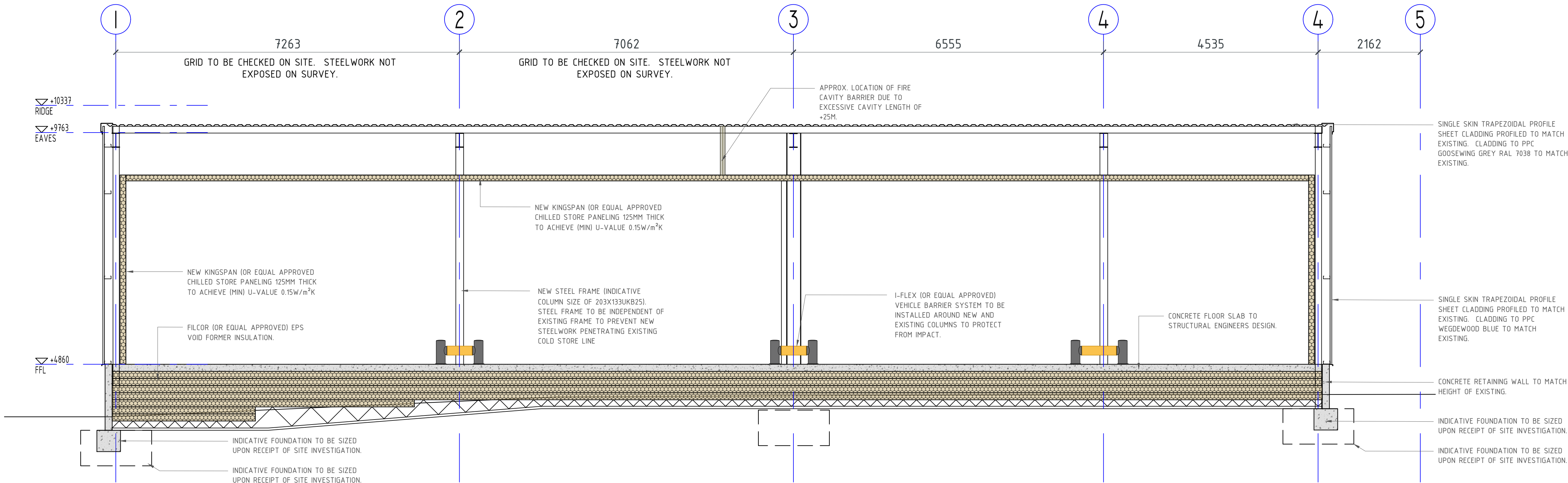
SECTION A-A SCALE 1:50@A1
