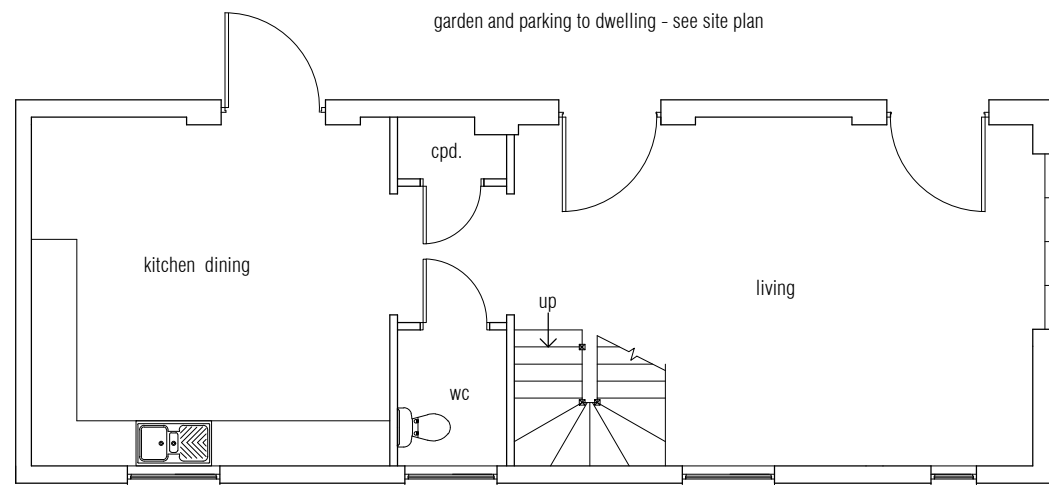
Ground Floor 1:50 scale
