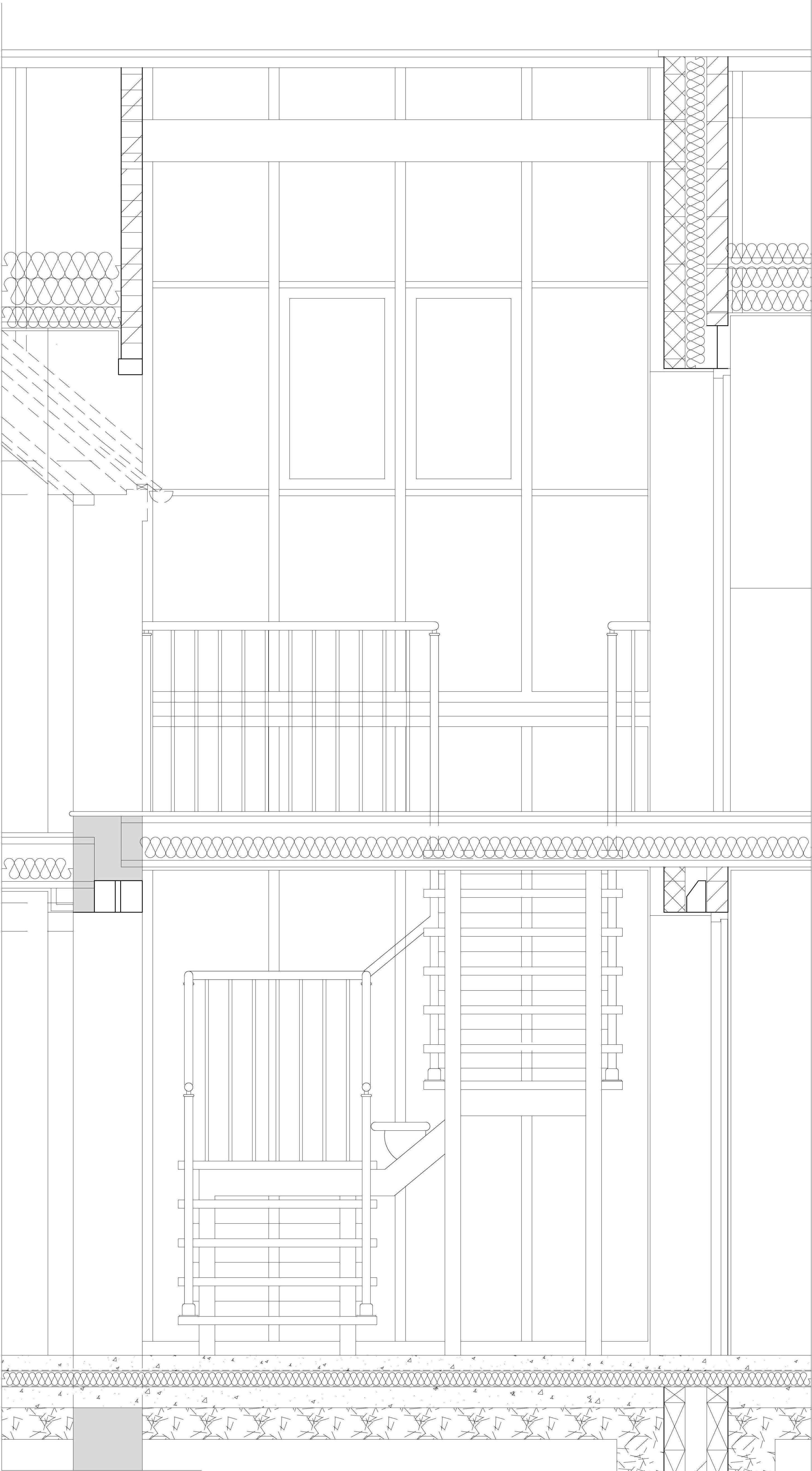
SECTION A - A
