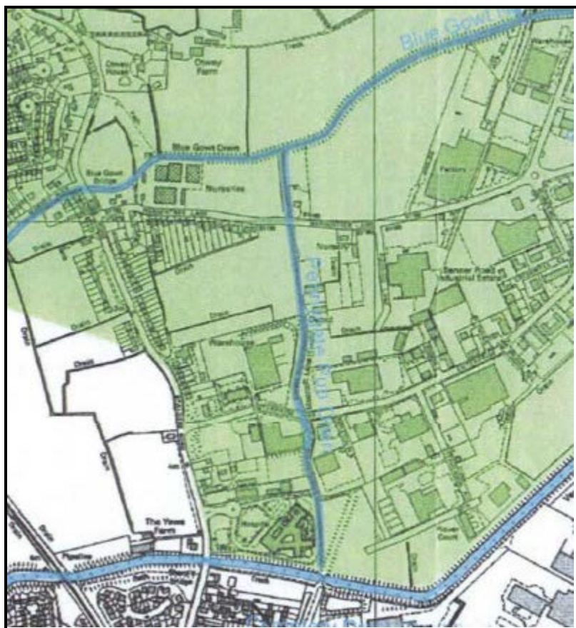
Extract from Welland and Deepings IDB Drainage Map
