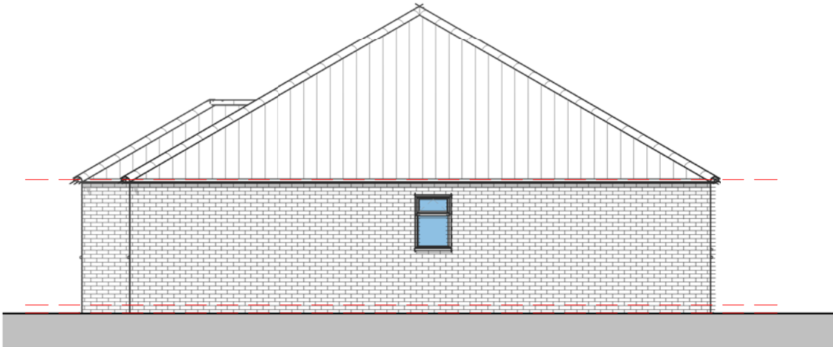
Elevation 02 – Right 1 : 100
