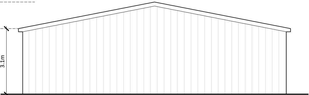
Side Elevation
