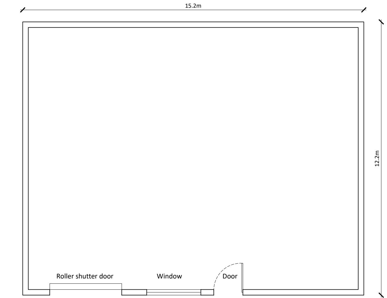
Floor Plan
