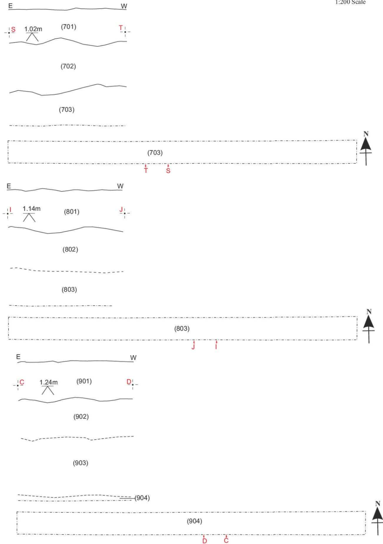
Figure 6: Trench plans (1:200) and sections (1:20)
