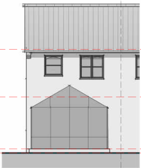
03 - Rear Elevation 1 : 100
